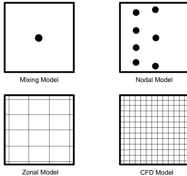
Figure 2.5 Room Air Model Classification (Chen and Griffith, 2002)
