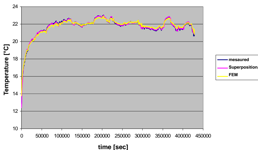
Figure 4: Measured temperatures, temperatures simulated with superposition method, and temperatures simulated with FEM of an instable test run (from Sauer, 2013)
