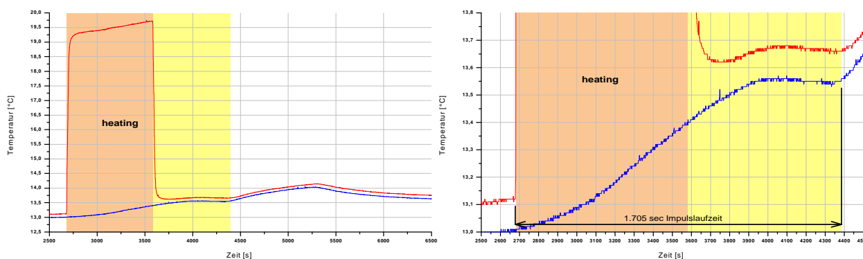
Figure 7: Principle of Thermo-Impulse method (recurrence of impulse), from Sauer & Sanner 2011).
