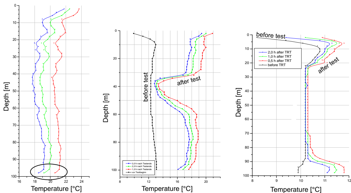
Figure 6: Temperature logs 1, 2 and 3 hours after a TRT in a relatively homogeneous lithology, showing the effect of “bottom heat dissipation” (encircled in black, left); a zone of high groundwater flow elucidated by temperature logs (centre), and a BHE with grout missing over a certain depth range (right), from Sauer & Sanner (2011).
