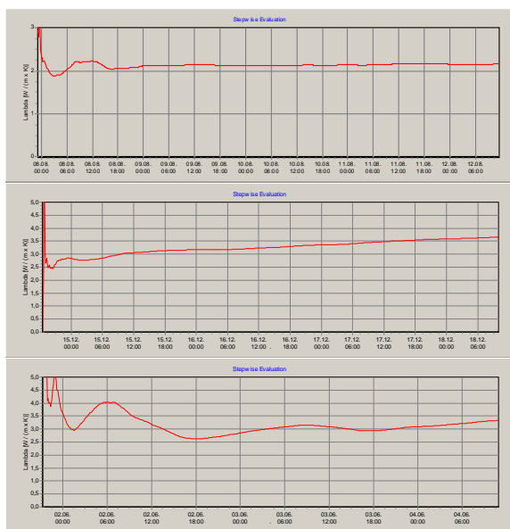
Figure 5: Sequential evaluation of TRT showing a stable result (top), a steady increase of thermal conductivity over test time (groundwater influence, centre) and erratic variations (e.g. due to power fluctuations, bottom), from Sauer & Sanner (2011)
