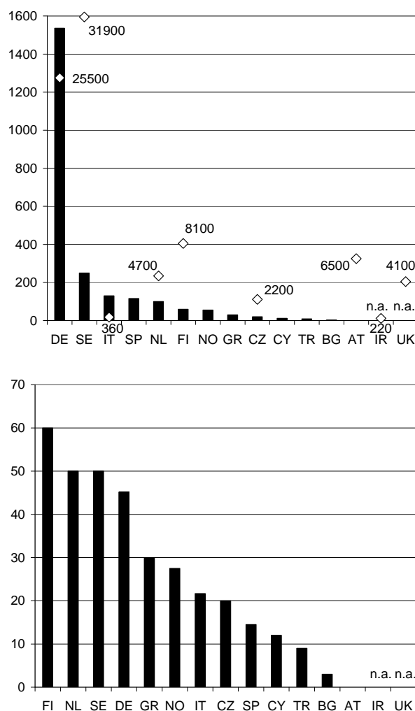
Figure 3: Total numbers of TRT performed in Europe (above, with some GSHP sales numbers for 2010 from EurObserv´er, 2011), and average number of TRT performed per rig in Europe (below), based on data sheets on IEA ECES Annex 21 website and some additions (status ca 2010).
