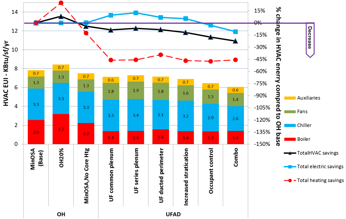
Figure 3: Energy performance comparison, Site HVAC EUI, Sacramento
