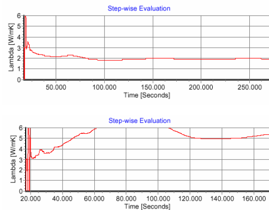
Figure 8: Step-wise evaluation showing perfect convergence (above) and test with high groundwater flow (below) and unreasonably high thermal conductivity value (data courtesy of UBeG GbR. Wetzlar)
