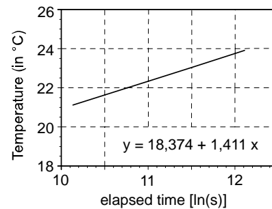
Fig. 6: Regression curve of mean fluid temperature in Thermal Response Test in Langen 1999
