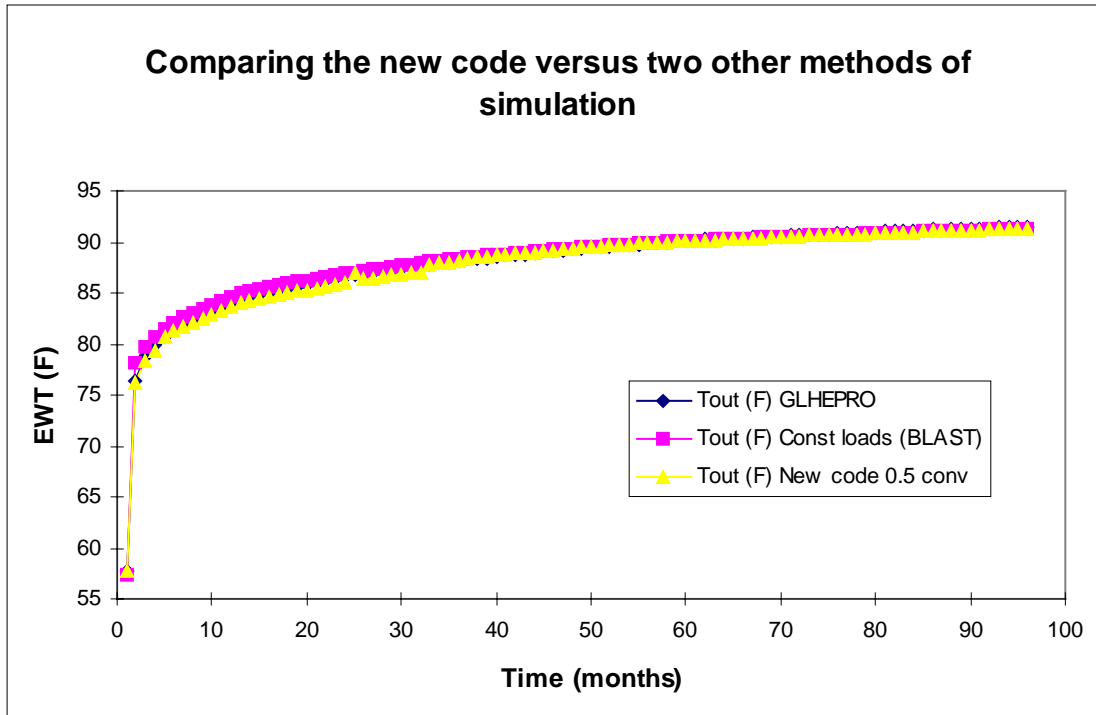
Figure 3.6 Comparing all three methods of simulation.
