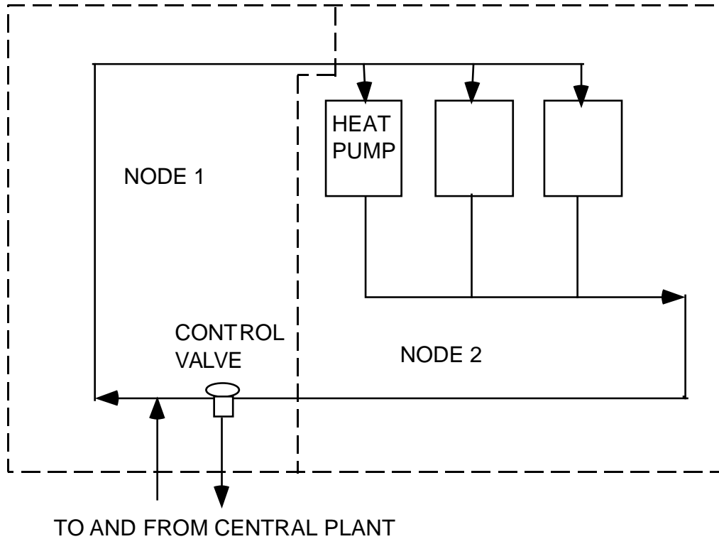
FIGURE 1.4 WATER LOOP
