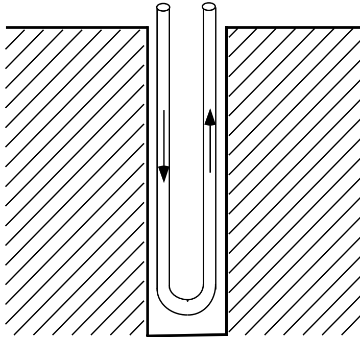
Figure 1.1 Closed loop vertical borehole
