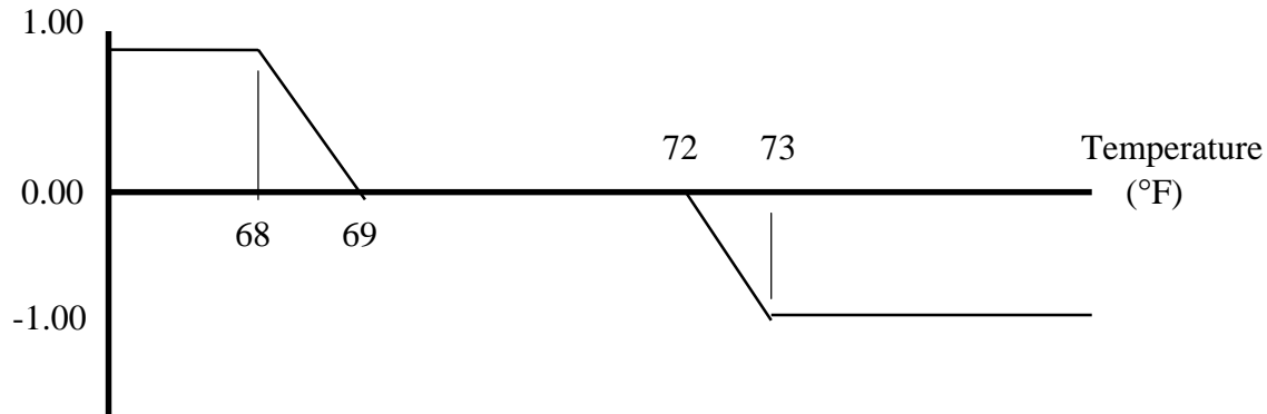
Figure 3.8 Occupied Control Profile.
