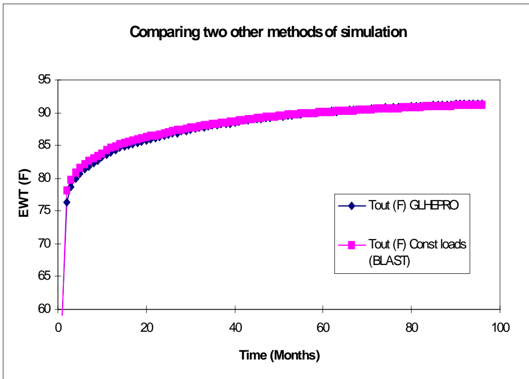
Figure 3.5 Comparing the GLHEPRO Model with the Constant Loads Model.
