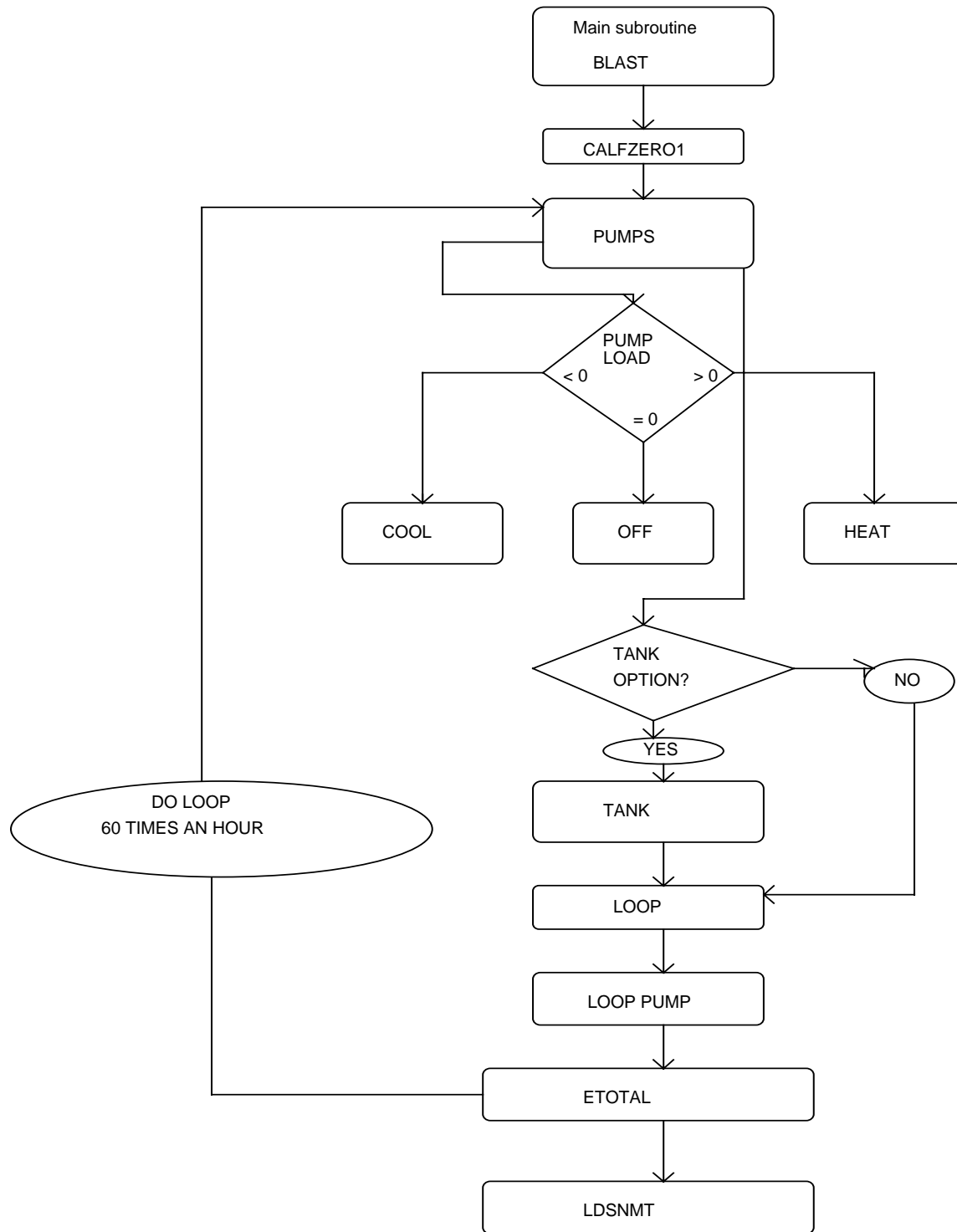
FIGURE 1. SUBROUTINES CALLED DURING RUNNING WLHPS IN BLAST
