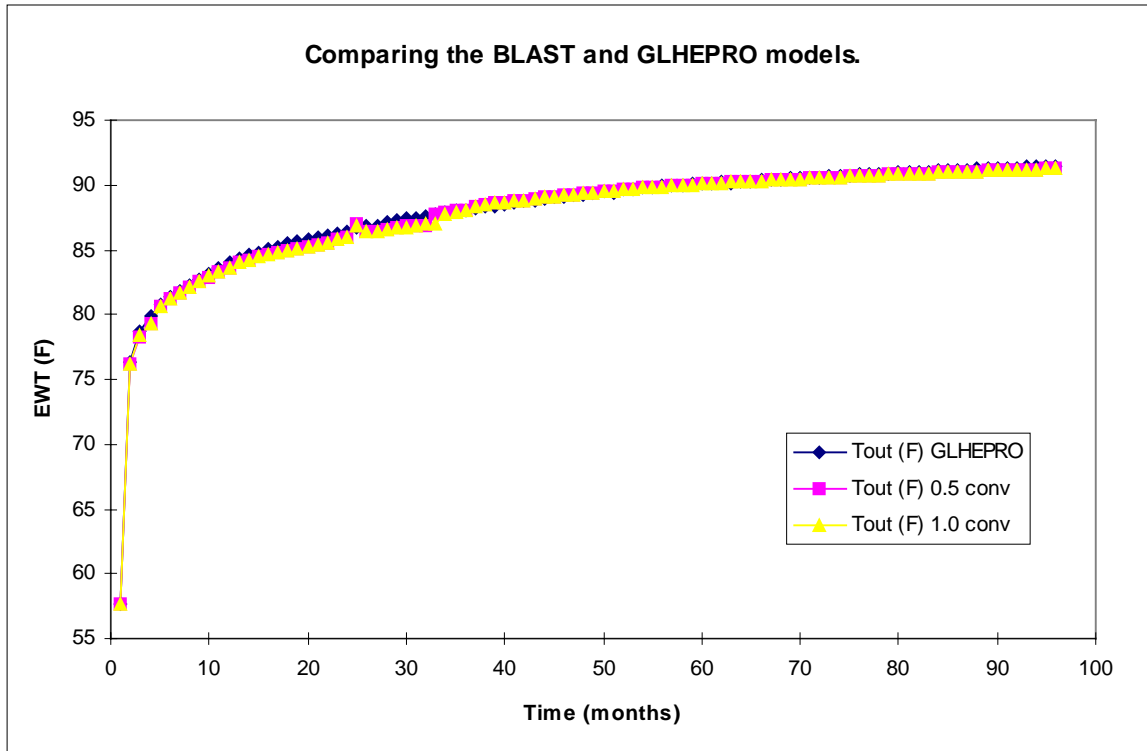
Figure 3.4a Comparing the BLAST and GLHEPRO Models
