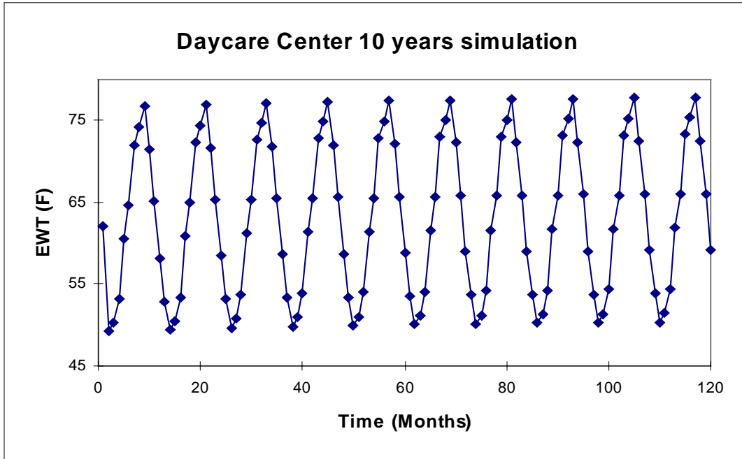
Figure 3.11 Heat Build Over a Ten Year Period for the Daycare Center
