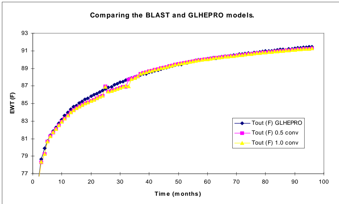
Figure 3.4b Comparing the BLAST and GLHEPRO Models
